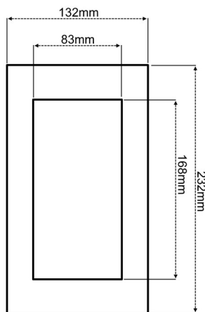
VDT-821/3x1 (3 modul)
